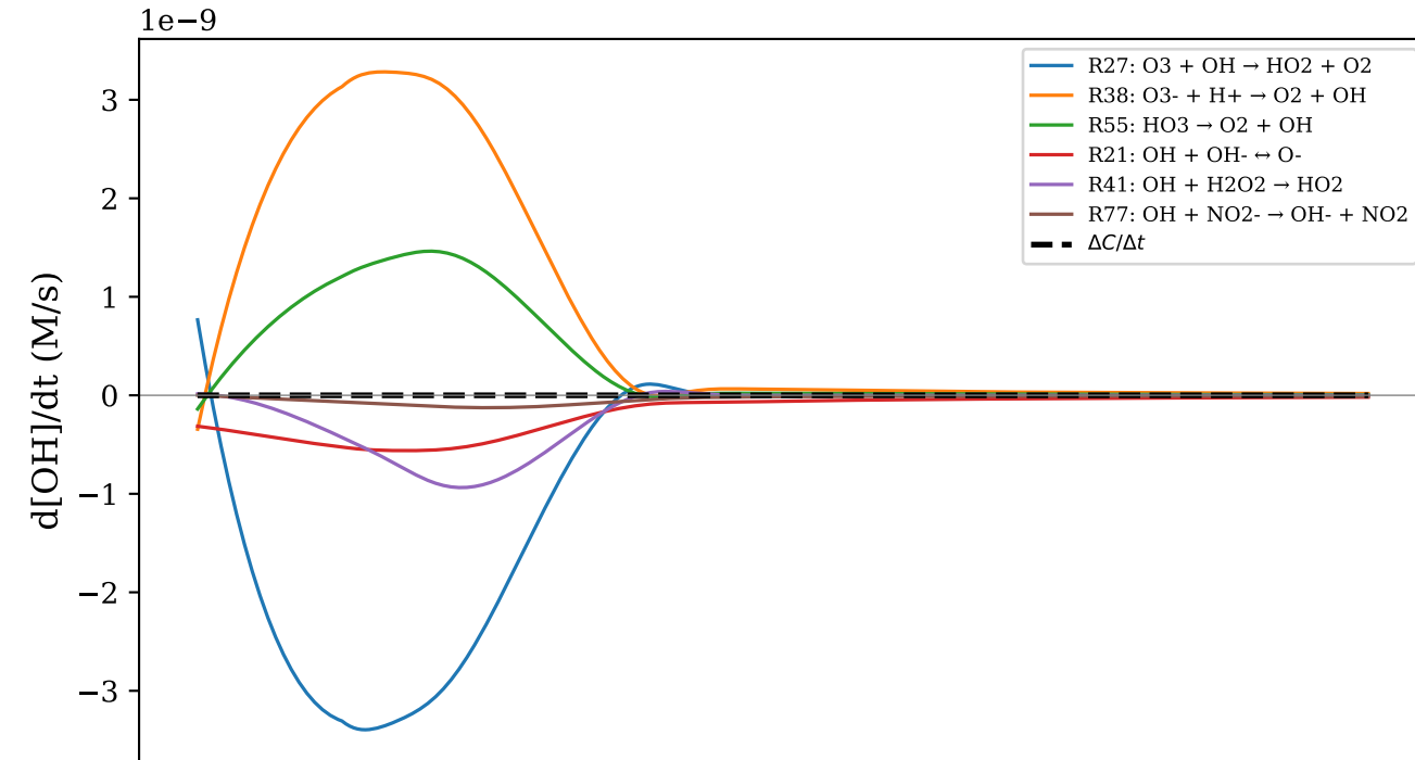
(b) OH [final=0.04 pM]
