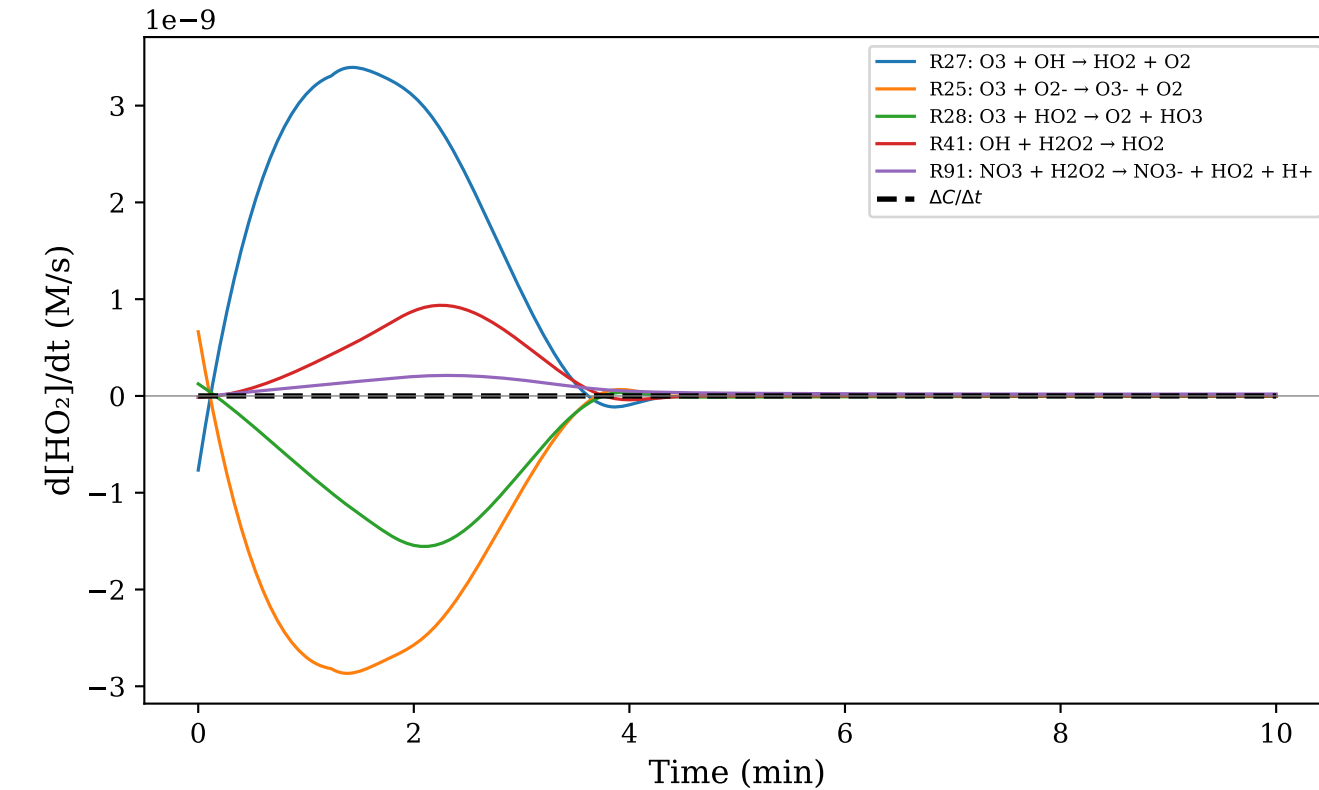
(c) HO 2 [final=1.12 pM]
